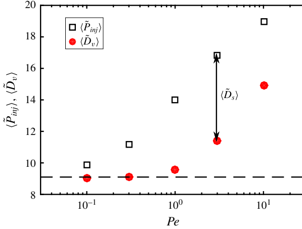
FIGURE 10. (Colour online) The temporally averaged viscous dissipation \langle \tilde{D}_v \rangle (red circles) and the injected power \langle \tilde{P}_{inj} \rangle (black squares) as a function of the Péclet number for Ca = 0.1 and Bi = 1 . The dashed line corresponds to the injected power \langle \tilde{P}_{inj} \rangle for the case without surfactants.
